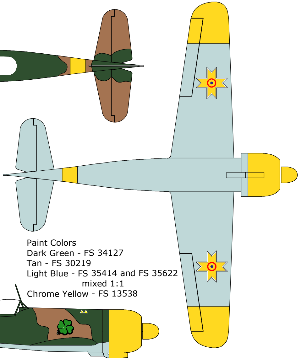
IAR-80 flown by Locotenent aviator Ion Galea of Escadrila 47, Grupul 9 Vinotar (Fighter), April 1942
